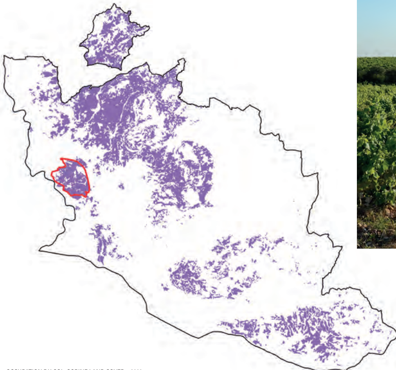
OCCUPATION DU SOL, CORINE LAND COVER - 2006
